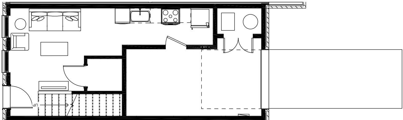
1ST FLOOR
